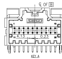
20PIN
