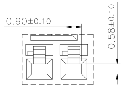
DETAIL A 4:1
